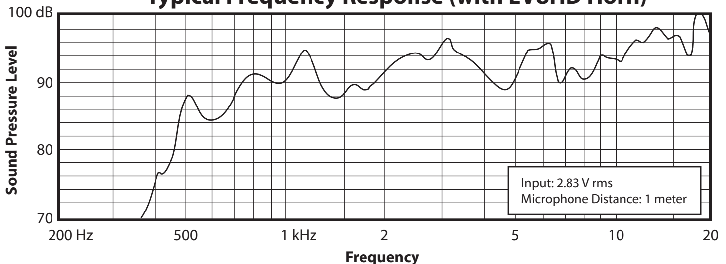
Typical Frequency Response (with EV8HD Horn)
